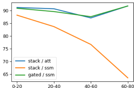
Figure 6: Accuracy by binned length on QNLI.
