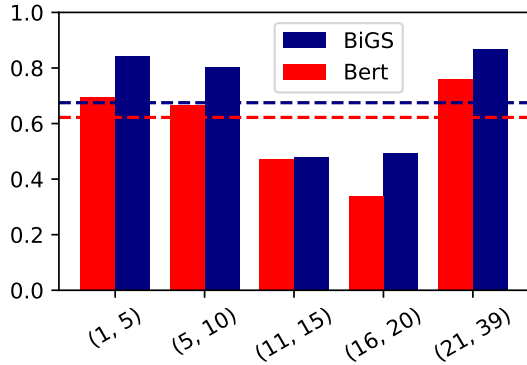
Figure 7: Performance of CoLA w.r.t sentence length using matthews correlation coefficient(MCC). The red and navy dashed lines in the graph represent the mean value obtained from multiple rounds of evaluation.
