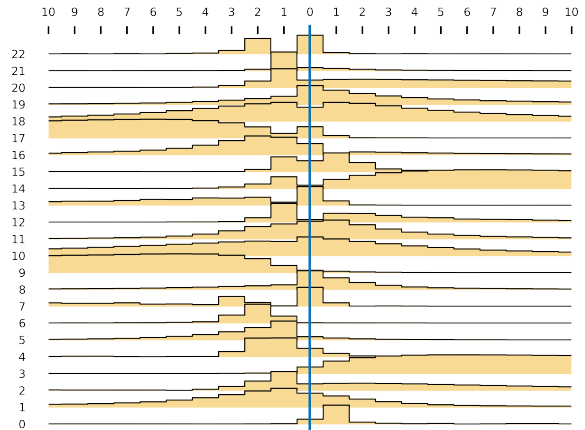
Figure 3: Complete SSM routing learned in BiGS. Shows forward and backward kernels \bar{\mathbf{K}} at each layer (0-22). Values indicate absolute value of contribution of each relative position (-10, \dots, 10) cropped from the full 2 \times 128 . Min-max scaling of absolute values is used for visual normalization.
