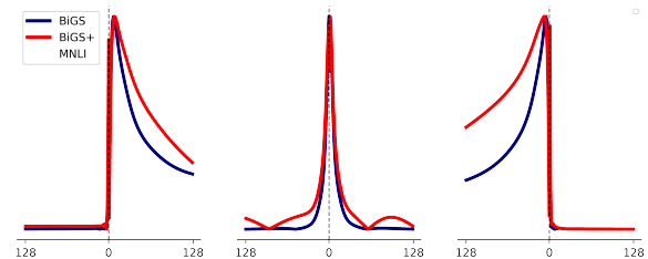
Figure 4: Change in SSM kernel after finetuning. Shows \bar{\mathbf{K}} after pretraining and after MNLI finetuning for Layer 14, Layer 18, and Layer 17 over all relative positions (-128, \dots, 128) .
