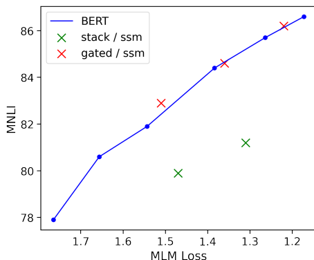
Figure 5: Comparison of pretraining loss and downstream accuracy. Plots MNLI accuracy with respect to MLM loss. BERT values from (Devlin et al., 2018). Gated SSM shows similar transferability as BERT, whereas Stack SSM does not.
